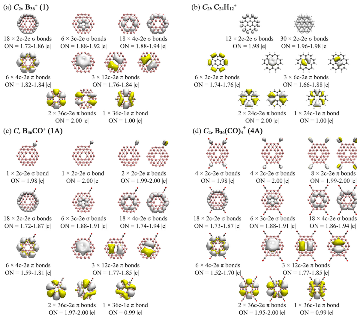
Fig. 3 AdNDP bonding patterns of (a) C_{2v} B_{36}^+ (1) , (c) C_s B_{36}(CO)^+ (1A) , and (d) C_{2v} B_{36}(CO)_4^+ (4A) compared with that of coronene monocation (b) C_{2h} C_{24}H_{12}^+ , with the occupation numbers (ONs) indicated and the \sigma -lone pairs on O atoms omitted.
