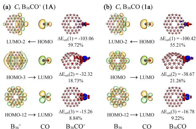
Fig. 5 Plots of the deformation densities \Delta\rho and shapes of the most important interacting orbitals of the pairwise orbital interactions between (a) \text{B}_{36}^+ and CO in \text{C}_5\text{B}_{36}\text{CO}^+ ( 1A ) and (b) \text{B}_{36} and CO in \text{C}_5\text{B}_{36}\text{CO} ( 1a ), with the orbital interaction energies \Delta E_{\text{orb}} (in kcal mol -1 ) and their percentage contributions to the overall orbital interactions indicated. The color code of the charge flow is from red to blue.
