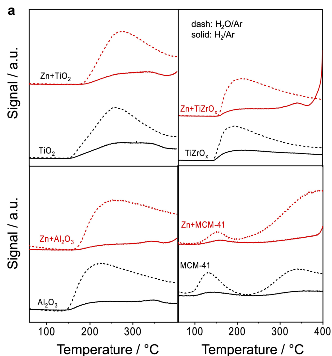
Extended Data Fig. 8 | \text{ZnO}_x species formation over different metal oxides. a , Concentration profiles of \text{H}_2 and \text{H}_2\text{O} detected by an on-line mass spectrometer upon temperature-programmed heating of bare supports or
