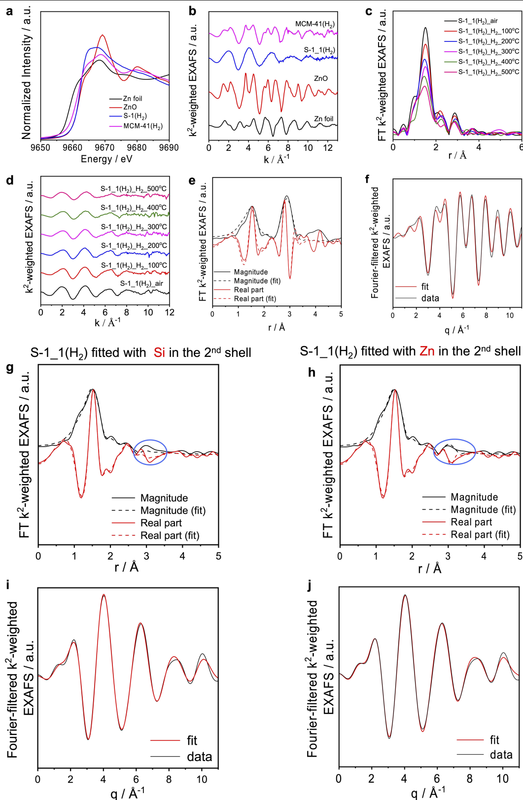
Extended Data Fig. 2 | Ex situ, in situ XAS and fitting data. a. XANES spectra of as-prepared catalysts and reference materials (Zn foil and commercial ZnO). b. The corresponding k^2 -weighted \chi(k) functions (extracted fine structure in k space) to a. c. In situ FT EXAFS spectra of S-1_1(H 2 ) in a flow of 5vol% H 2 in He at different temperatures. d. The corresponding k^2 -weighted \chi(k) functions (extracted fine structure in k space) to c. e. f. The EXAFS fits of the ZnO reference (used to estimate amplitude reduction factor) in r (e) and q spaces (f). ZnO fit summary (based on the wurtzite structure): \delta E_0 = 1.0 \pm 2.6 eV; \rho = 2.0\% ;
