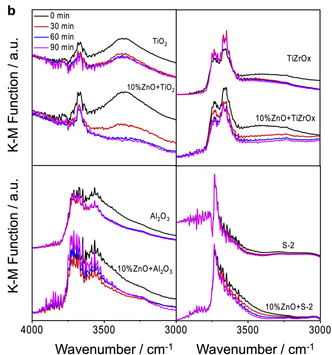
physically mixed metallic \text{Zn}^0 and a certain support in Ar. b , In situ DRIFTS spectra of bare supports or a mixture of \text{ZnO} with a certain support. Reaction conditions: 550^\circ\text{C} , 50vol% \text{H}_2 in Ar.
