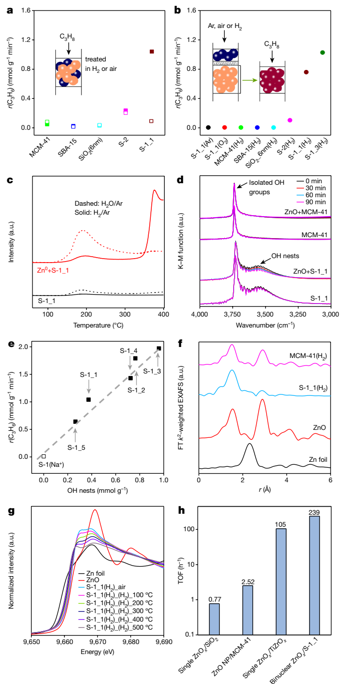
Fig. 1 | Catalyst activity, formation of ZnO x species and their structure. a , r(\text{C}_3\text{H}_6) at 550 °C over oxidatively (open symbols) or reductively (closed symbols) treated mixtures of ZnO (blue spheres) and SiO 2 -based support (orange spheres). b , r(\text{C}_3\text{H}_6) over Zn-containing materials (dark-red spheres), prepared as shown in the inset. c , H 2 and H 2 O evolution upon temperature-programmed heating of a mixture of Zn 0 and S-1_1 in Ar. d , In situ DRIFTS spectra of S-1_1, MCM-41, or their mixtures with 10wt% ZnO at 550 °C in H 2 /Ar = 1. e , r(\text{C}_3\text{H}_6) over reduced ZnO-silicalite-1 at 550 °C versus the concentration of OH nests in differently prepared silicalite-1. f , Ex situ FT EXAFS spectra (not corrected for the phase shift) of different materials. g , In situ XANES spectra of S-1_1(H 2 ) treated in 5vol% H 2 in He at different temperatures. h , Turnover frequency (TOF) of propene formation over Zn-based catalysts. The values of single ZnO x /SiO 2 and single ZnO x /TiZrO x are reported in ref. 19 and ref. 24 , respectively.
