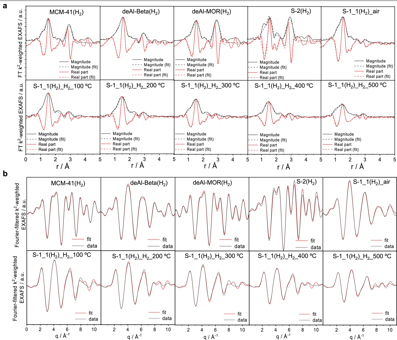
Extended Data Fig. 3 | Fitting results. a, b, The EXAFS fits for different materials in r ( a ) and q spaces ( b ).
