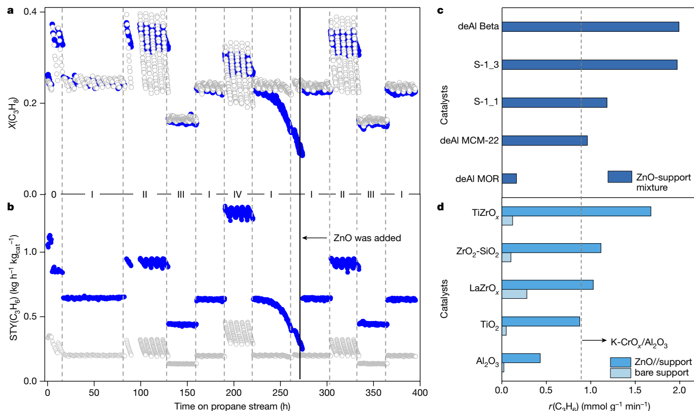
Fig. 3 | Durability test and validation of the approach. a, b, On-stream profiles of X(\text{C}_3\text{H}_8) (a) and \text{STY}(\text{C}_3\text{H}_6) (b) over ZnO//ZnO-S-1_3 (blue, 0.09 g of ZnO and 0.09 g of ZnO-S-1_3) and K-CrO x /Al 2 O 3 (grey, 0.302 g). Only the amount of ZnO-S-1_3 was considered for calculating \text{STY}(\text{C}_3\text{H}_6) . Reaction conditions: 550 °C, (I): \text{C}_3\text{H}_8:\text{H}_2:\text{N}_2 = 4:2:4 , 10 or 6 \text{ml min}^{-1} , (II): \text{C}_3\text{H}_8:\text{H}_2:\text{N}_2 = 4:2:4 , 6 \text{ml min}^{-1} , (III): \text{C}_3\text{H}_8:\text{H}_2:\text{N}_2 = 4:4:2 , 6 \text{ml min}^{-1} , and (IV): \text{C}_3\text{H}_8:\text{H}_2:\text{N}_2 = 7:3 , 6 \text{ml min}^{-1} . c, d, r(\text{C}_3\text{H}_8) over ZnO-zeolite mixtures (reduced for 1 h) (c) or ZnO/metal oxides (reduced for 2 h) (d). A scheme of reactor loading for c, d is present in Extended Data Fig. 7e and 7a, respectively.
