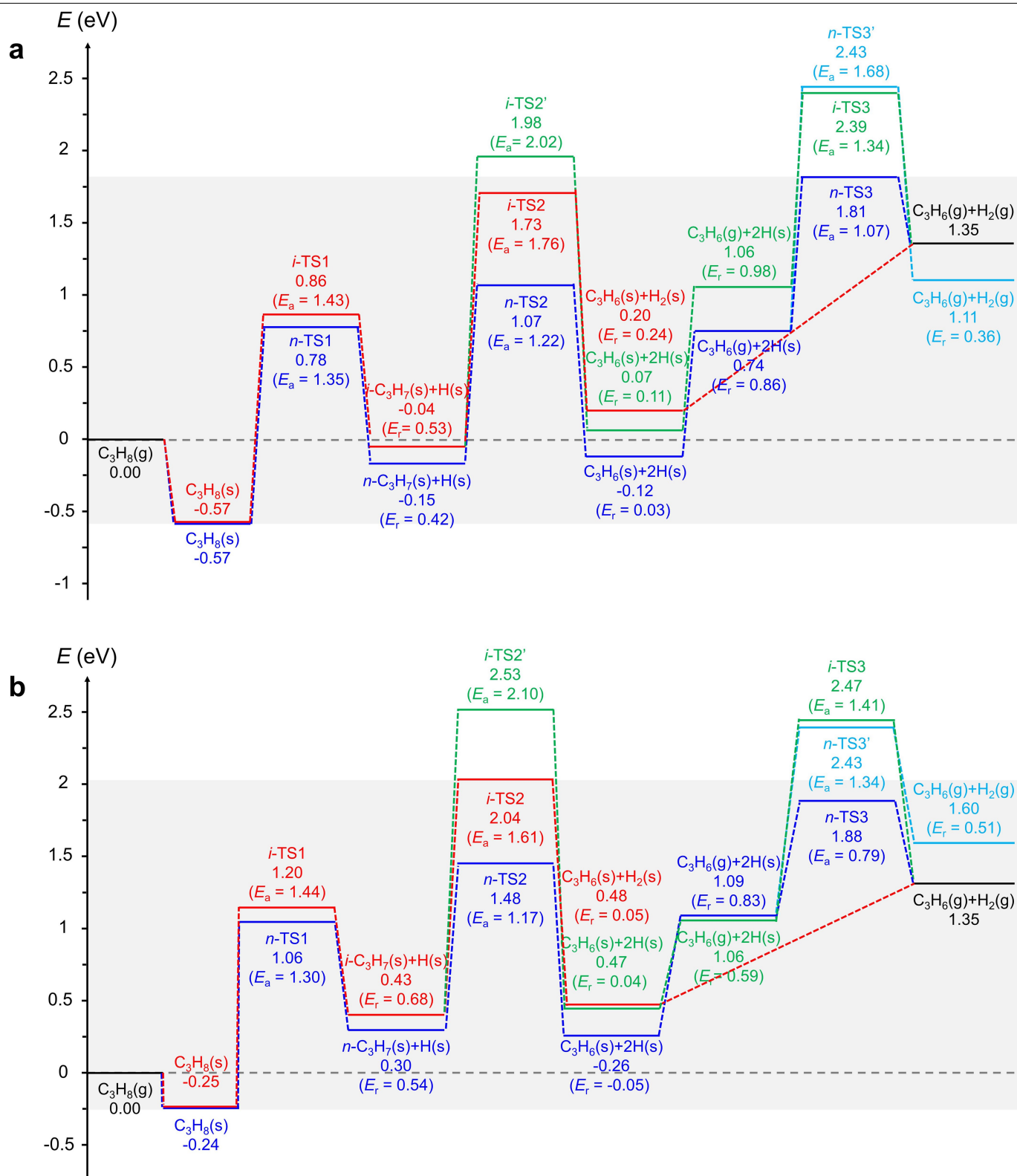
Extended Data Fig. 6 | Potential energy surface of different reaction pathways in PDH. a, The potential energy surface of PDH using the binuclear ZnO_x/S-1 model at the PBE + D3 + ZPE level. Two competitive PDH paths are considered: (i) propane is initially activated upon methyl C-H heterolytic cleavage to yield n-C_3H_7 or (ii) propane is activated at the central methylene
