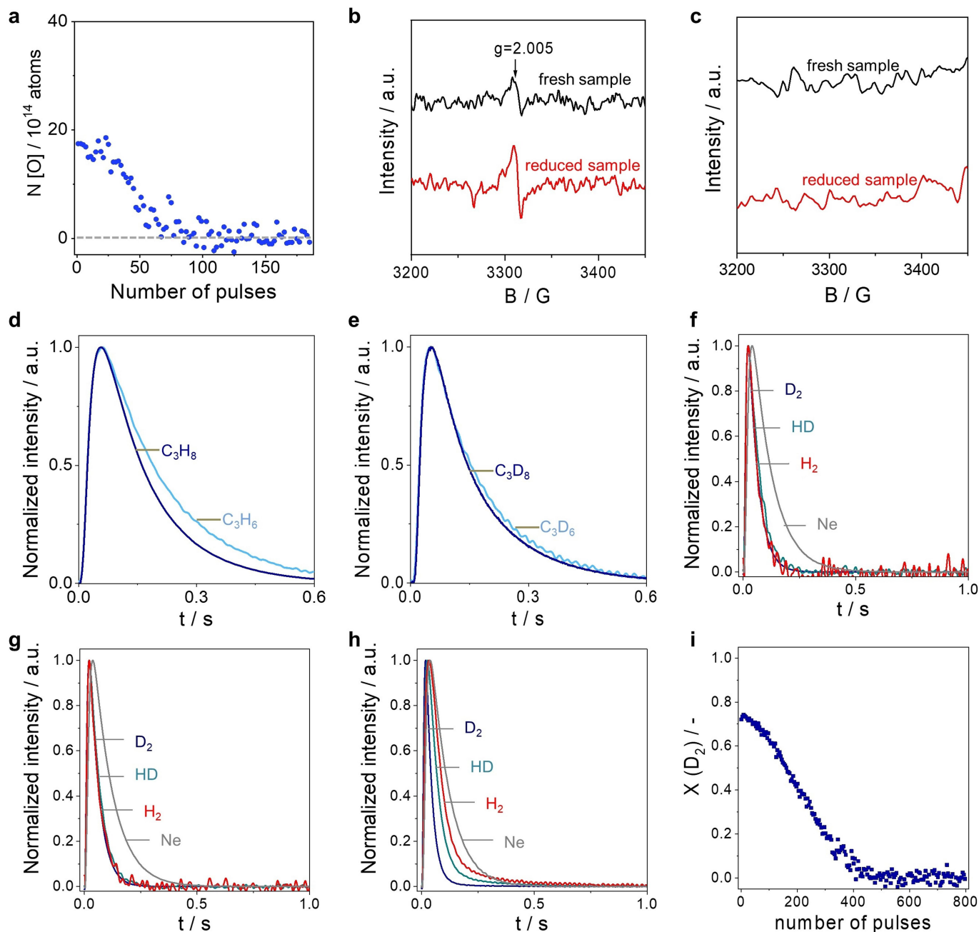
Extended Data Fig. 4 | Proving the presence of O vacancies and rate-limiting step in PDH. a , The amount of consumed oxygen atoms ( N[O] ) upon O_2 pulsing at 550 °C over S-1_1( H_2 ) reduced in H_2/Ar = 1 at 550 °C for 0.5 h. b, c , In situ EPR spectra at 20 °C of fresh and treated ( H_2/Ar = 1 (20 ml min -1 ) at 550 °C for 1 h) S-1_1( H_2 ) ( b ) or bare S-1_1 ( c ). d, e , Height-normalized transient responses of C_3H_8 , C_3H_6 , C_3D_8 , C_3D_6 , D_2 and HD recorded after pulsing of
