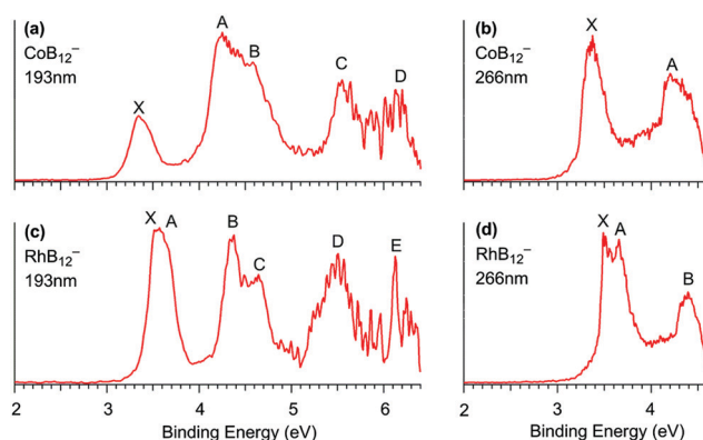
Fig. 45 Photoelectron spectra of CoB_{12}^- (a and b) and RhB_{12}^- (c and d) at 193 nm and 266 nm. Reproduced from ref. 88 with permission from the American Chemical Society, copyright 2014.
